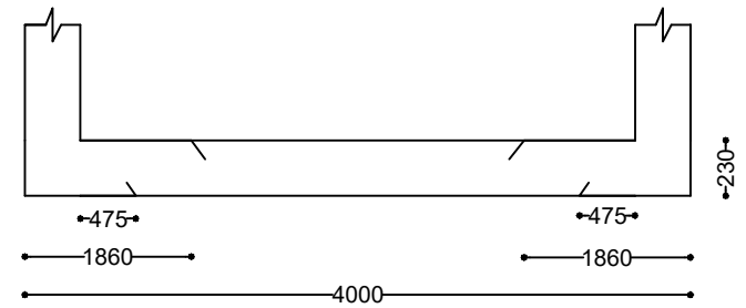
BEAM DETAILS
