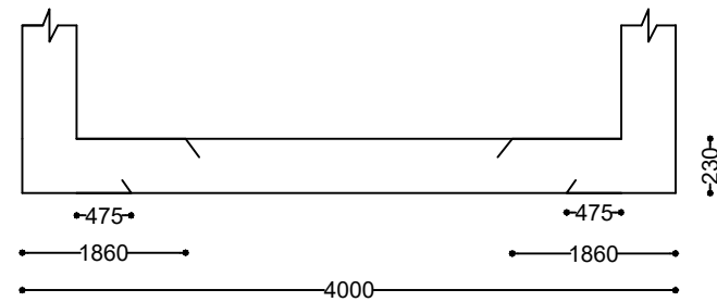
BEAM DETAILS
