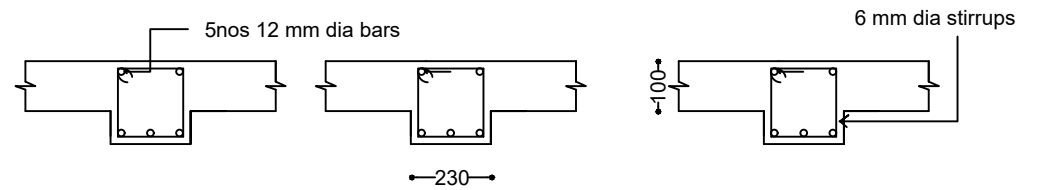
CROSS SECTION OF BEAM
