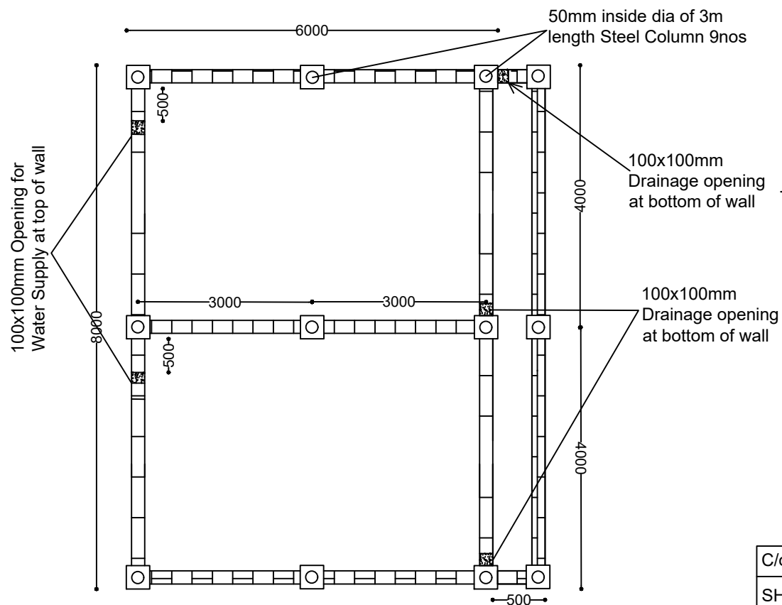
PLAN VIEW
