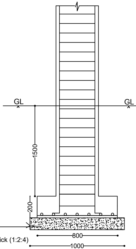
FOOTING DETAILS
