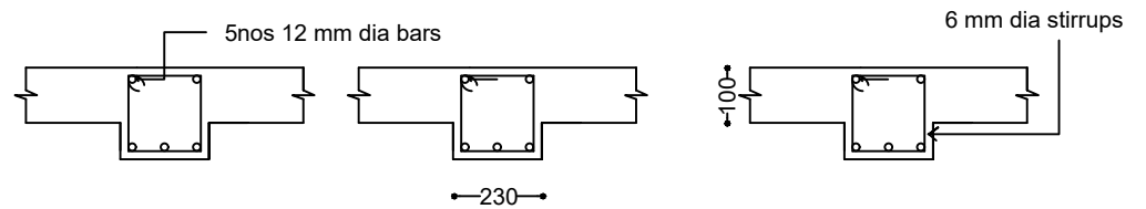
CROSS SECTION OF BEAM
